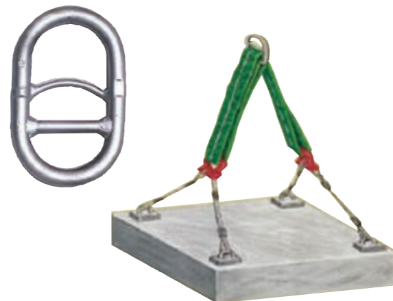
Twin-Path® adjustable bridles self adjust over the centre of gravity.
